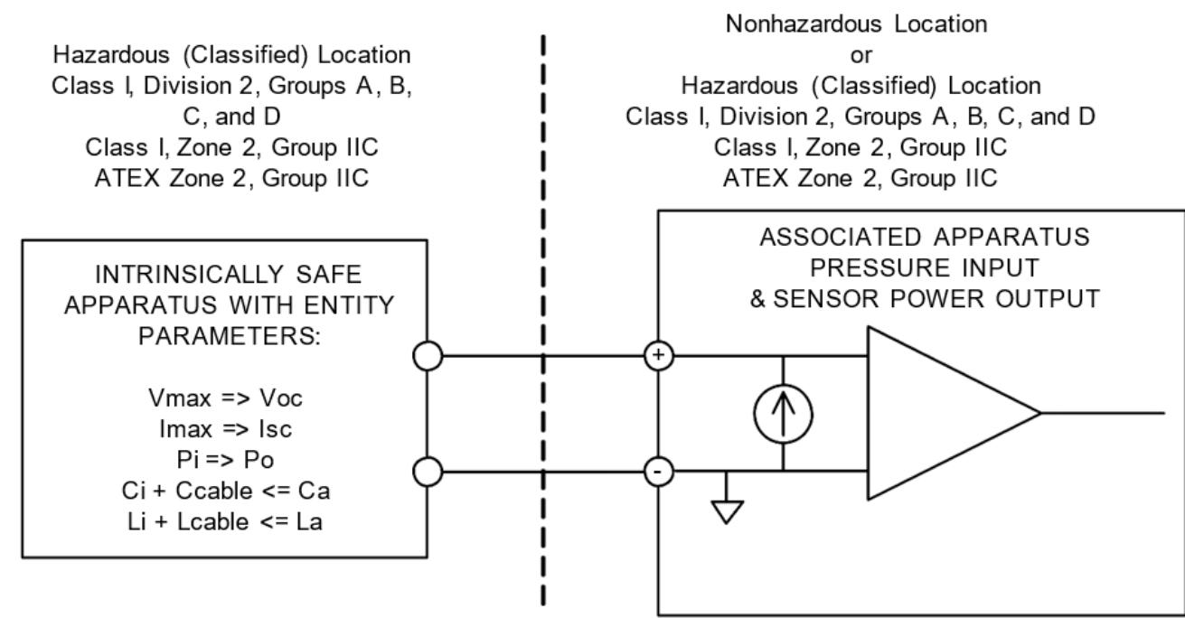
Wiring Diagram
