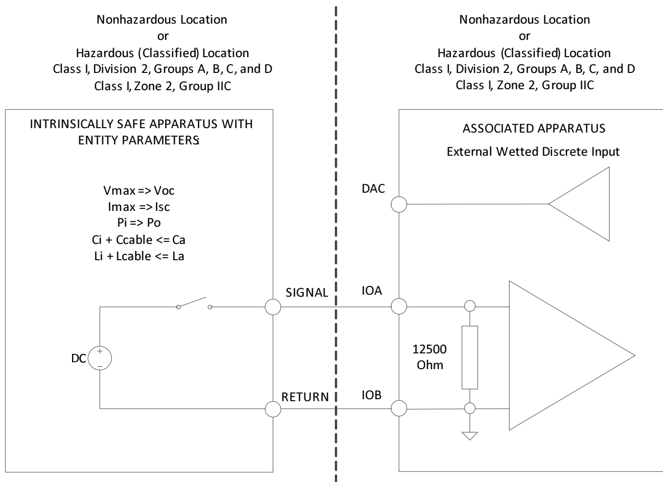
Wiring Diagram
