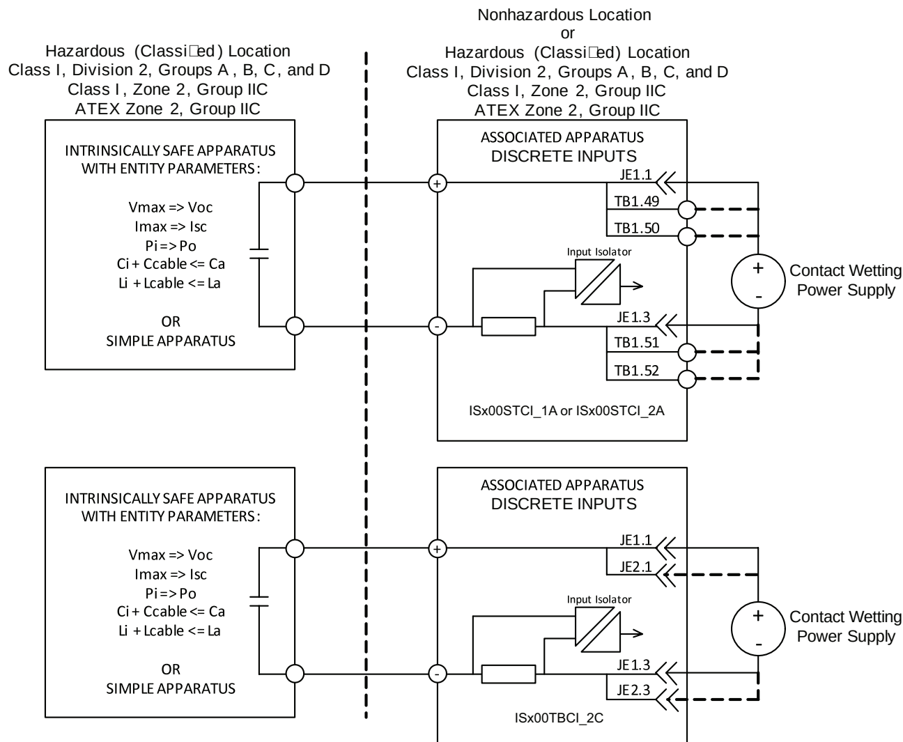
Wiring Diagram
